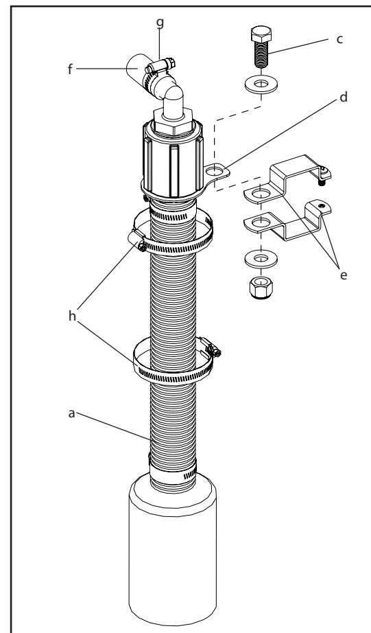
Figure 4: Discharge Tube
