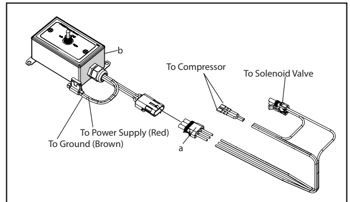
Figure 2: Wiring harness
